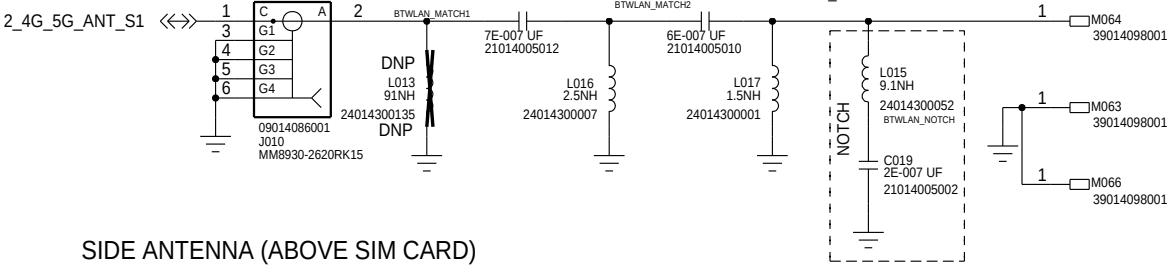
BT/WLAN CHAIN0 ANTENNA REF:010-019
